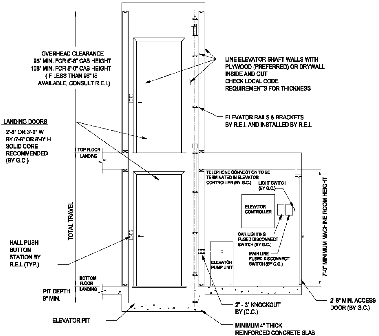
TYPICAL ELEVATION AND LAYOUT (ADJACENT MACHINE ROOM)
